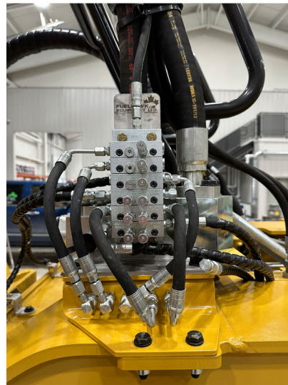
Custom Bolt on bracket designed to fit specifically on this unit
